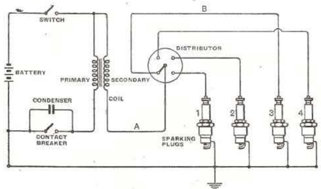
Fig. 2.—A conventional ignition circuit without suppression.
