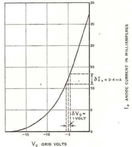
Fig. 2.—The slope (mutual conductance) of a valve curve depends on the point selected. An approximate result is given by measuring (by meter or from the graph) the change in current due to a change in voltage near that point. It would be 2.4 mA/V in this example.
