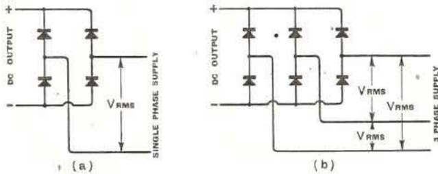
Fig. 2.—A single-phase full-wave bridge connected rectifier is shown in diagram (a); the addition of two rectifying limbs, as in diagram (b), results in a three-phase rectifier of the same type.
