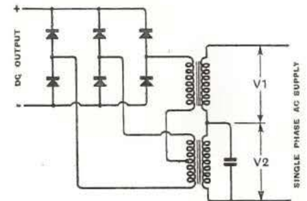
Fig. 5—Fundamental circuit of the new constant potential system. A phase-splitting circuit is used on the primary side, and the transformer secondary windings are Scott-connected to provide a three-phase supply to the rectifier at full load. Variations in load current or supply voltage result in phase swinging which controls the DC voltage within fine limits.
